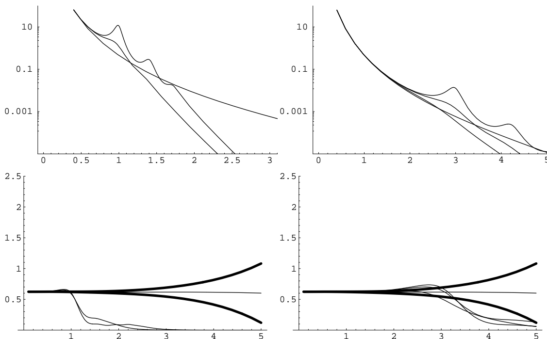
Figure 9: In the upper plots d\sigma/dM_{jj} (units of pb/GeV) vs M_{jj}(TeV) is plotted for the case of SM QCD background(thicker curve), and a toy stringy behavior with M_s=1 TeV in the lefthand plot with \gamma = .1, .3 and M_s=3 TeV in the righthand plot with \gamma = .1, .3, .6 . In the lower two plots the R_\eta is plotted for the same parameters.
