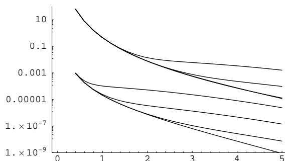
Figure 13: In the left panel d\sigma/dM (units of pb/GeV) vs M_{jj} (TeV) is plotted for QCD(the lowest curve) and a set of four fermion operators with \Lambda = 1, 2, 4 TeV. In the right panel R_\eta is plotted for the same operators as well as QCD with the statistical error bars for QCD are overlaid for 1 \text{ fb}^{-1} of data.
