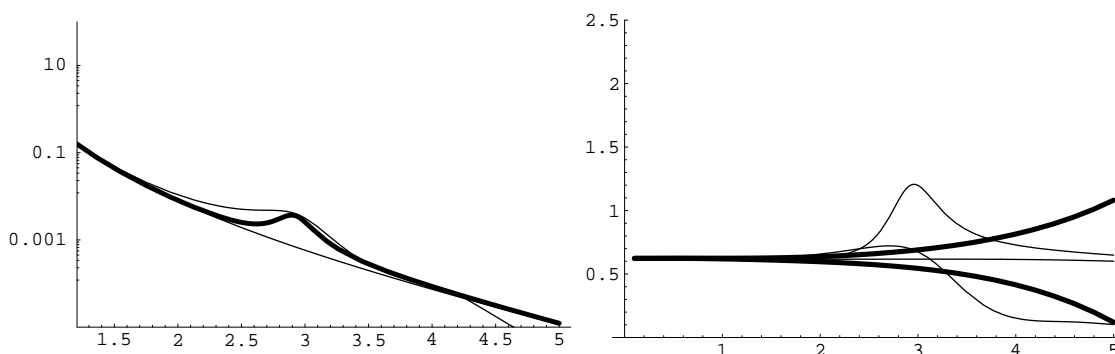
Figure 10: R_\eta is plotted for M_s = 1 TeV and \gamma = .1 for the amplitude defined with (4.5) with one sigma gaussian error bars corresponding to 1 inverse femtobarn of luminosity.
