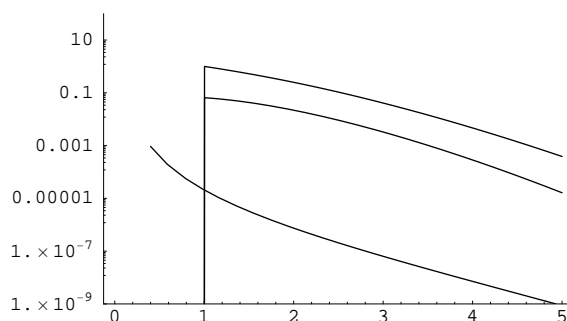
Figure 15: d\sigma/dM (units of pb/GeV) vs two body invariant mass(TeV). The curves from top to bottom represent black hole cross section for M_D = 1 TeV , n = 6 , and x_{\min} = 1 for a black hole decaying into l^+l^- (assuming any initial gauge charge is radiated softly), black hole cross section for M_D = 1 TeV and x_{\min} = 1 for a “charged” black hole decaying into l\nu , and the lowest curve is the Drell Yan background.
