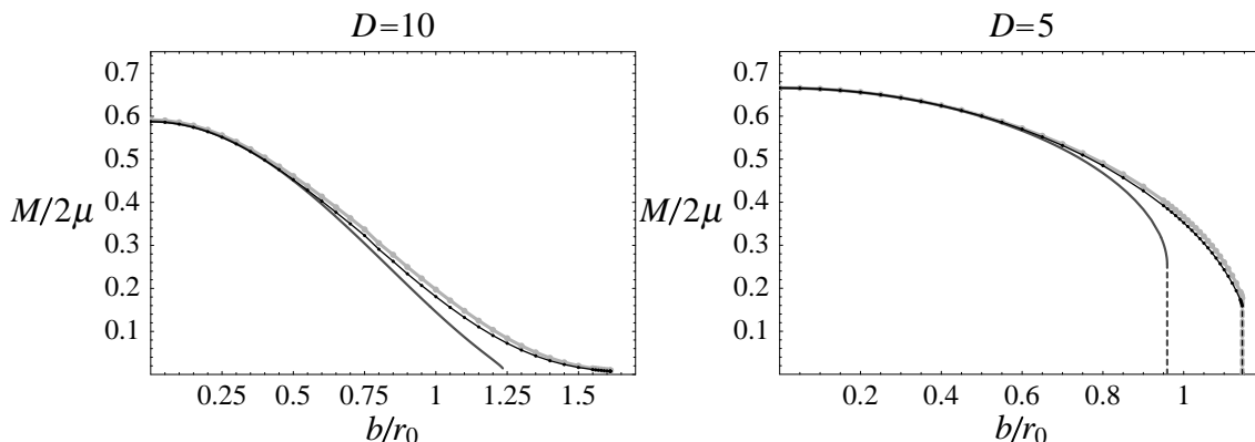
Figure 3: From figure 10 of [26]. The ratio of the mass of the putative black hole compared to the initial energy of the collision is plotted as a function of the impact parameter divided by a unit r_0 that approximates the Schwarzschild radius if all the energy of the initial collision were to end up as a black hole. The lowest curve represents the calculation of [26], and previous estimates from [24, 25] are also included.
